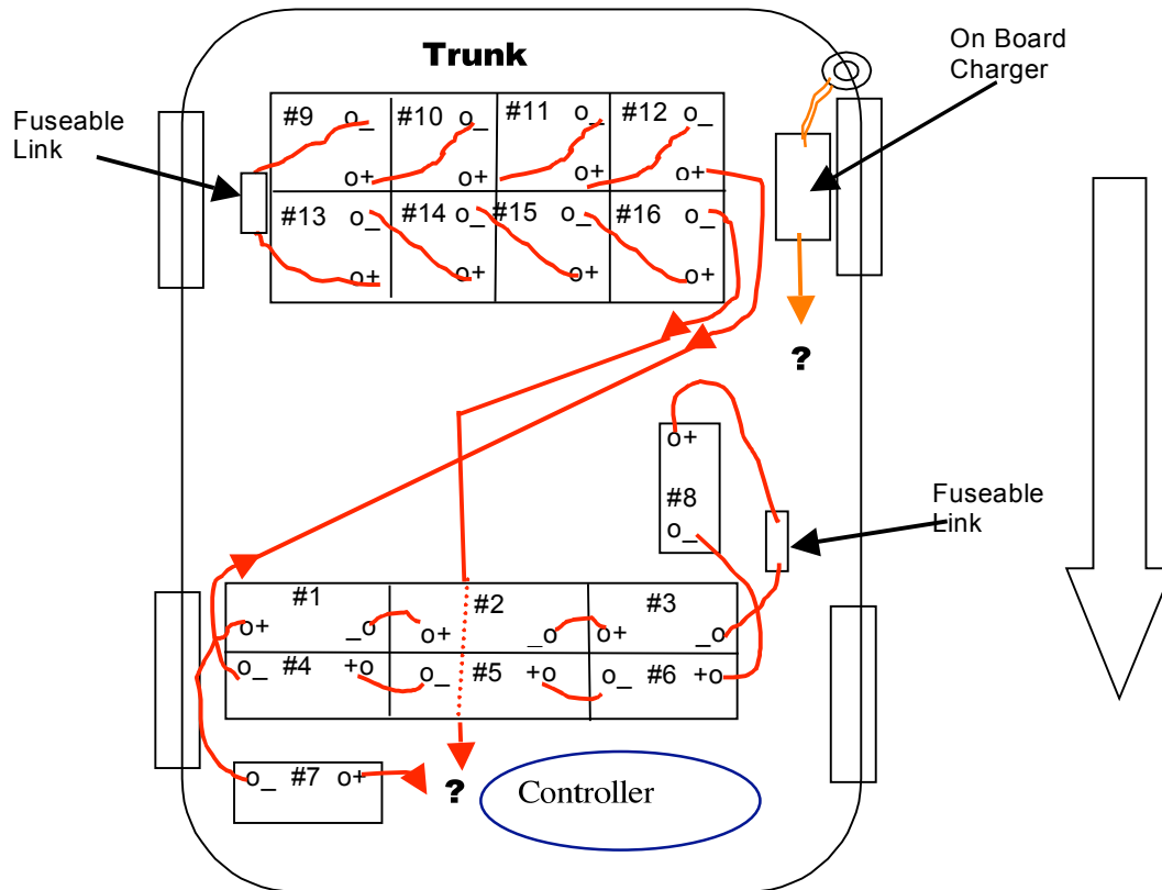
Figure 2. Battery Connections
